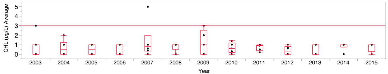
Figure 3. Plots of annual averages for total phosphorus, total nitrogen, total chlorophyll and Secchi disk visibility in Sugarloaf M-1 / Monroe County.
